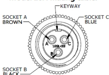
Model 20A mating cable:
